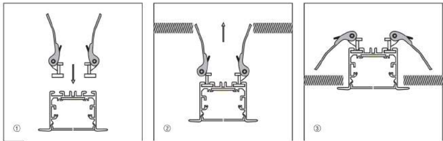
Clip Installed To Profile
