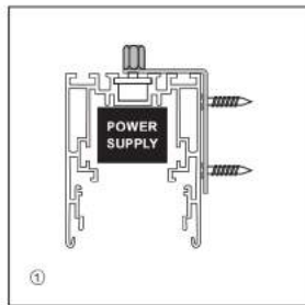
Installing profiles to wall
