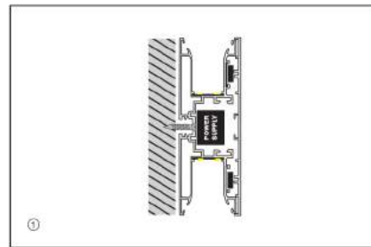
Installing profiles to wall
