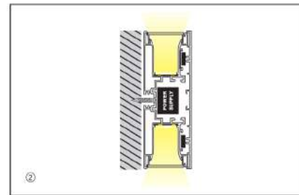
Installation of driver , light source pc cover and end cap Complete Fixed
