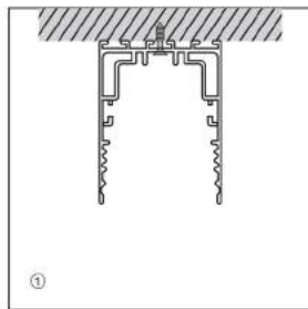
Installing profiles to ceiling
